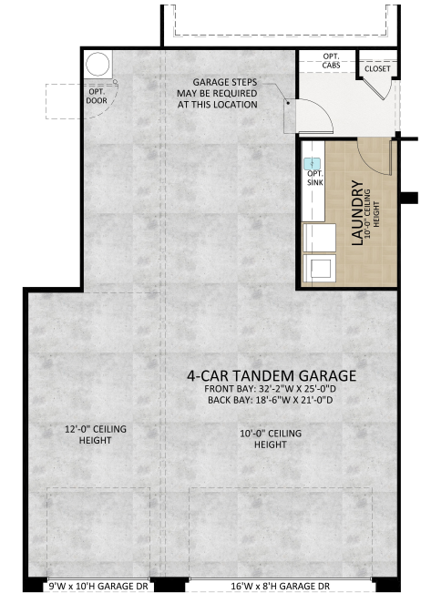
Optional Tall Garage At 4-car Tandem Garage
